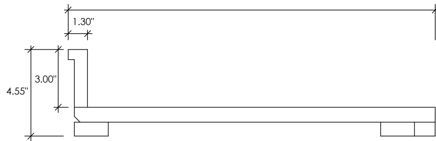
Countertop Detail
